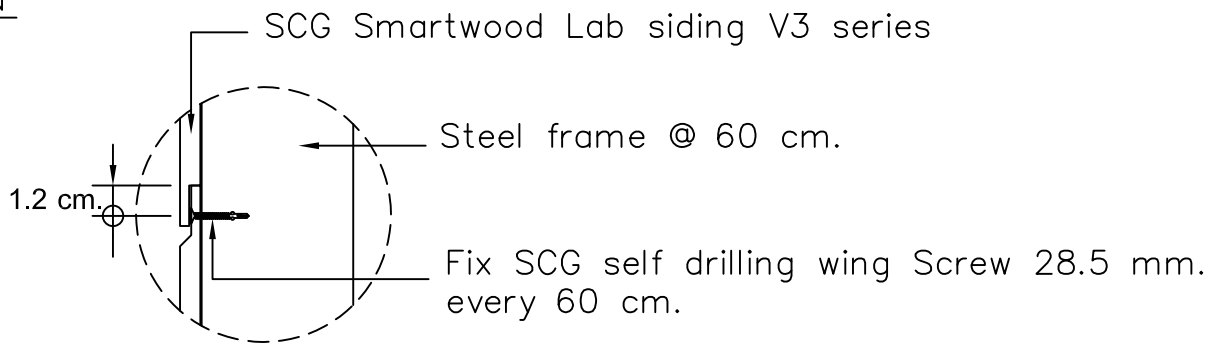
Detail A
